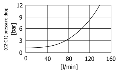
Oil supply flow (from C2 to C1)
