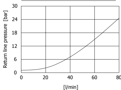
Flushing valve characteristic
